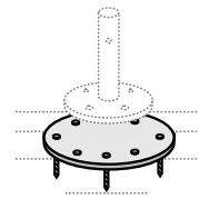
Base Plate 315mmø To bolt to concrete patio or wooden deck
